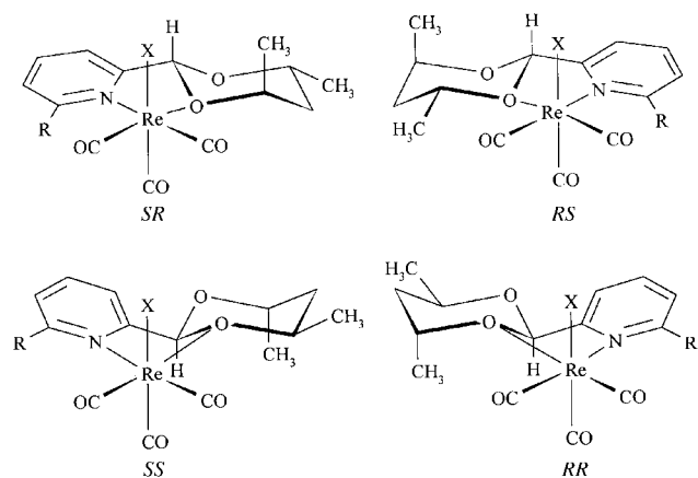
Fig. 2 The four possible diastereoisomers of the complexes [\text{ReX}(\text{CO})_3(\text{L})] ( \text{L} = \text{L}^1 or \text{L}^2 , \text{R} = \text{H} ; \text{L}^2 , \text{R} = (4R,6R)\text{-}4,6\text{-dimethyl-}1,3\text{-dioxan-}2\text{-yl} ). The letters refer to the configuration at the metal and the acetal carbon atom, respectively.
