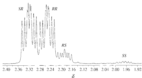
Fig. 4 Hydrogen-1 NMR spectrum of [\text{ReI}(\text{CO})_3(\text{L}^1)] in d_2 -tetrachloroethane, showing the signals due to \text{H}_D of the acetal ring. See Figs. 1 and 2 for labelling.
